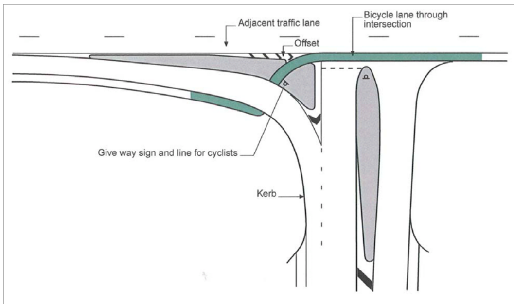
Figure 5.16: An example of provision for cyclists at rural free-flow left-turn treatments
