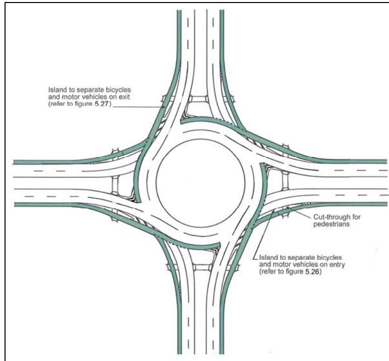
Figure 5.24: Bicycle lanes at a two-lane roundabout with physical separation for cyclists (some jurisdictions may not favour this treatment – see Section 5.5.1)
